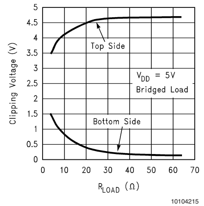
Clipping Voltage vs RL
